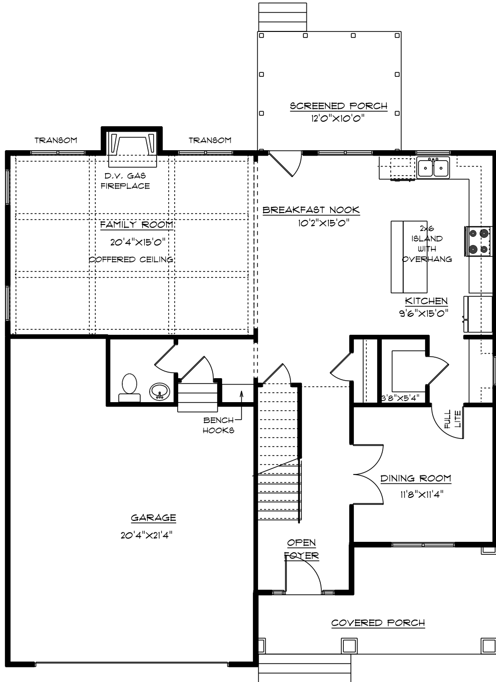
FIRST FLOOR PLAN CLARKSVILLE MODEL
