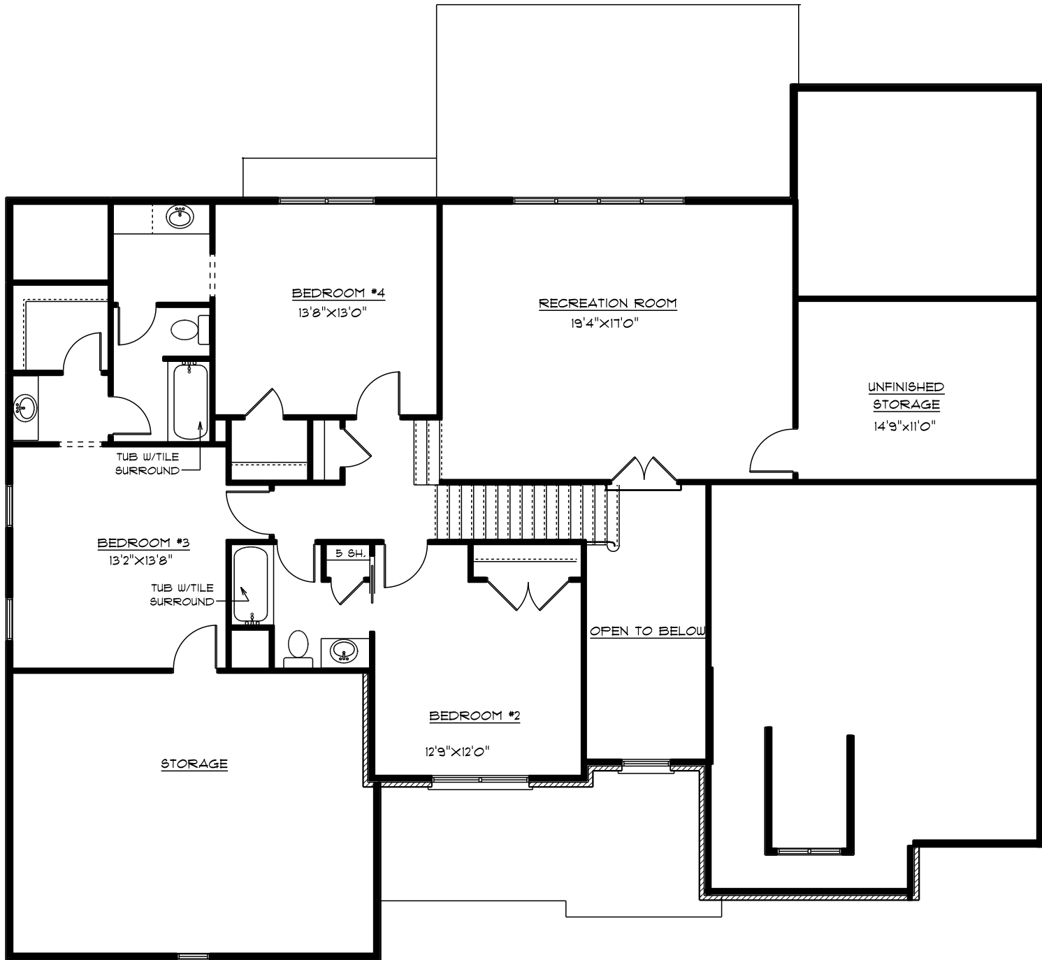
SECOND FLOOR PLAN GRAVES SPRINGS MODEL
