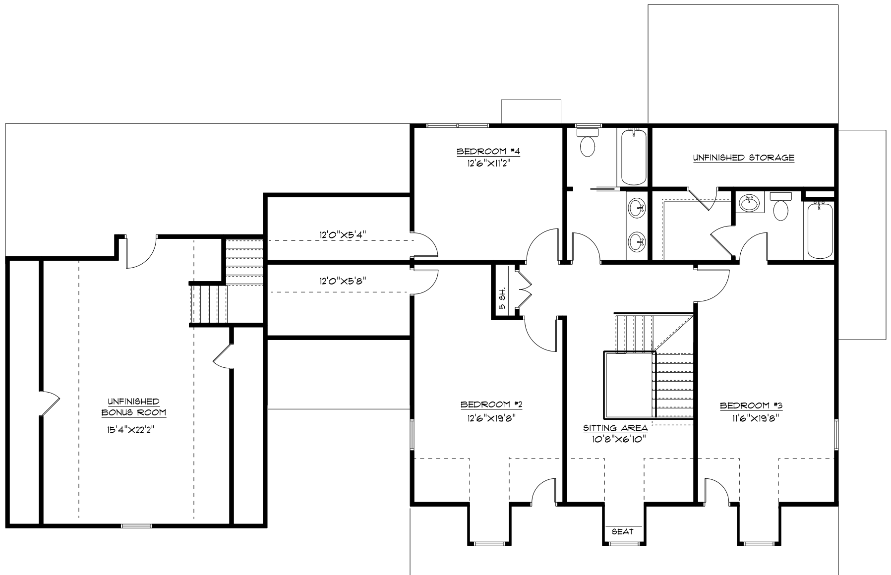
SECOND FLOOR PLAN THE MONTICELLO CAPE MODEL
