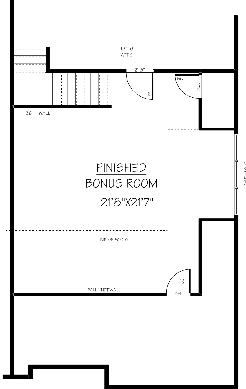
BONUS ROOM PLAN HARRISON PLACE MODEL
